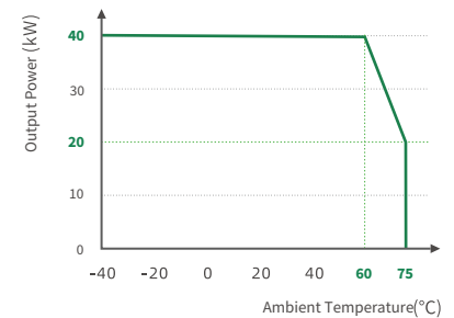
Temperature Characteristic Curve
