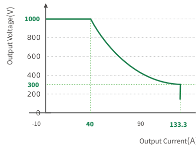
Output Characteristic Curve ( \leq 60^\circ\text{C} )
