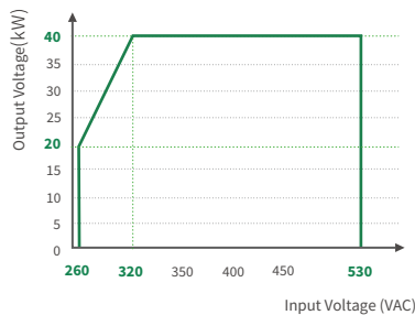
AC Input Characteristic Curve
